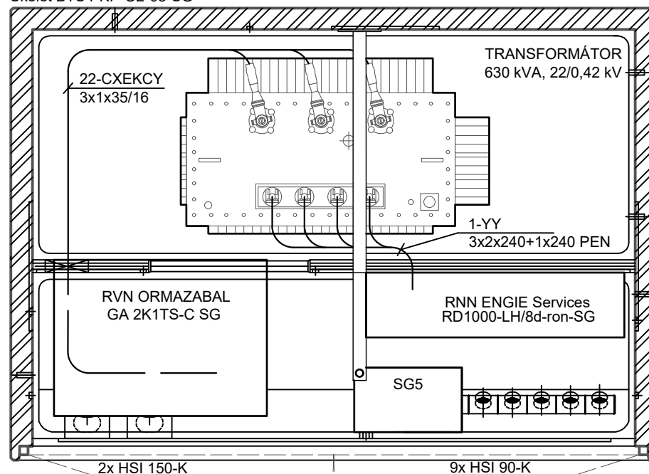
Skelet BTS PKP-O2-08-SG
