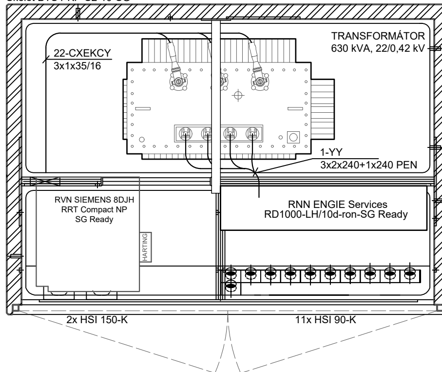
Skelet BTS PKP-S2-10-SG
